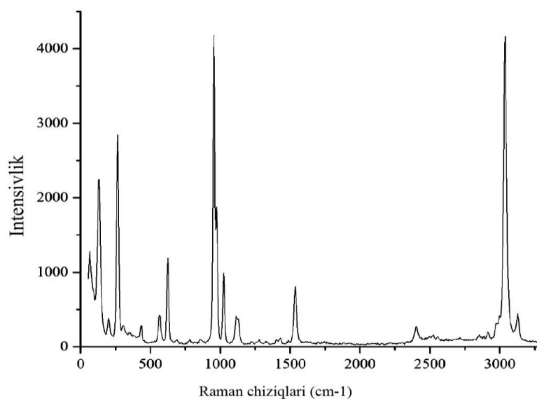
2-rasm. Suyuq brombenzolning Raman spektri
