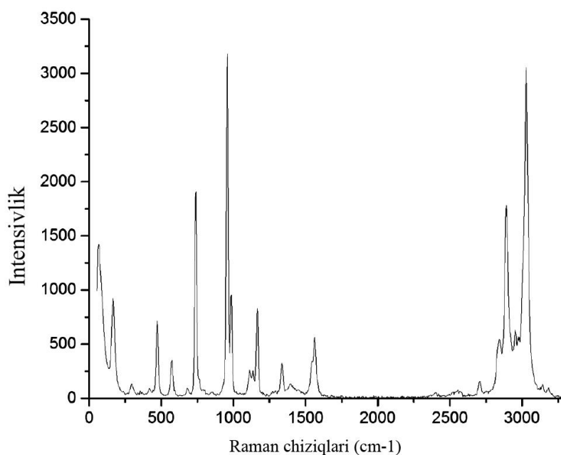
3-rasm. Suyuq toluolning Raman spektri
